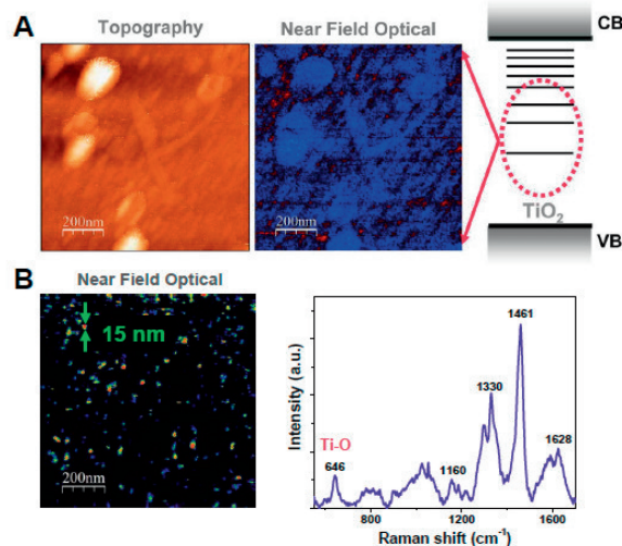
Figure 5. (A) Simultaneously obtained topographic and near field optical images of a clean Niobium-doped rutile TiO 2 (110) surface. Single surface states localized at the sub-domain boundaries can be clearly observed. (B) For the Alizarin adsorbed TiO 2 surface, resonance Raman spectrum (using 532 nm laser excitation) with the Ti-O peak at 646 cm -1 provides the evidence of the strong electronic coupling at the interface.
