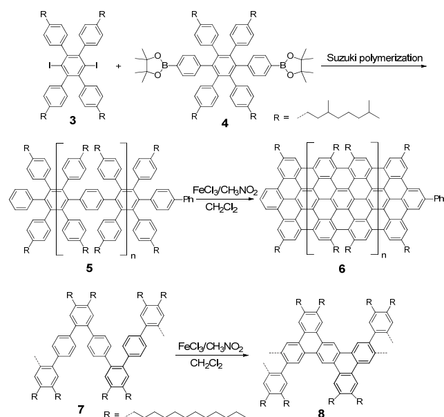
Scheme 3. Synthesis of linear ( 6 ) and kinked ( 8 ) graphene nanoribbons.
