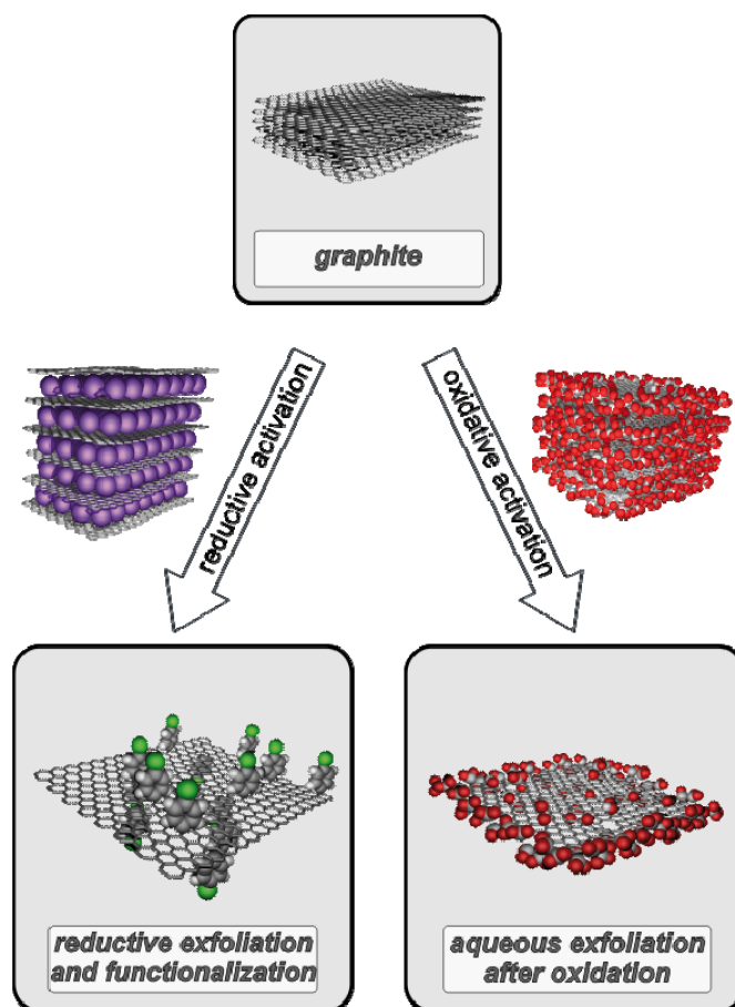
Figure 2. Covalently functionalized graphene by oxidation of graphite leading to graphene oxide (right) or via the recombination of potassium GICs with activated addends such as diazonium salts (left).
