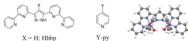
Figure 4. Left: bis(terdentate)X-Hbbp family of dinucleating ligands. Center: substituted monodentate pyridyl ligands. Right: calculated structure of a representative diruthenium complex, {[Ru II (py) 2 (H 2 O)] 2 (μ-bbp)} 3+ . Color code: Ru, pink; N, blue; O, red; C, gray; H, white.
