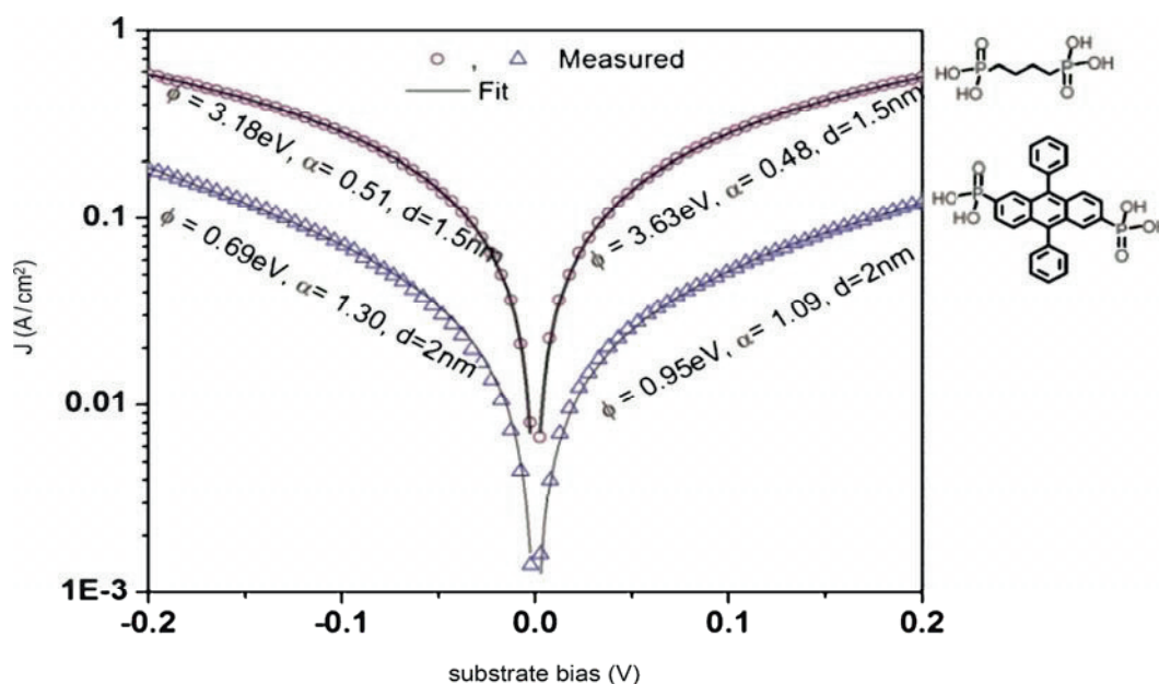
Figure 7. Absolute value of the current density as a function of substrate bias for 1,4-diphosphonobutane (top curve) and 9,10-diphenyl-2,6-diphosphonoanthracene ( 3 ) (bottom curve) SAMs on highly p-doped Si ( 10^{20} \text{ cm}^{-3} ). Open symbols are measured data and lines are model fits, with several of the fitting parameters displayed.
