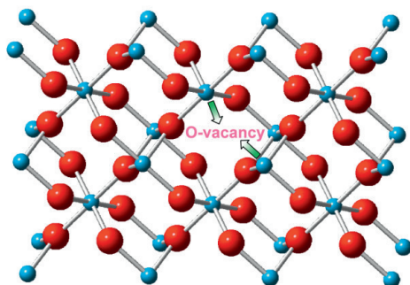
Figure 6. Conceptual view of the O-vacancy on rutile \text{TiO}_2 surface. The structure is plotted by ball and stick model (Red: O; Blue: Ti). Because there are two excess electrons occupying 3d orbital of two neighboring Ti atoms, two transition dipole moments will occur under laser excitation. The two arrows show the direction of the dipole moments.
