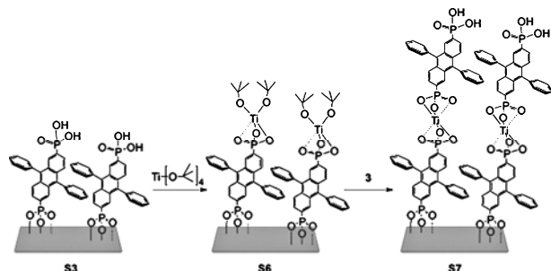
Figure 2. Synthesis of the duplex of 9,10-diphenyl-2,6-diphosphonoanthracene ( 3 ).
