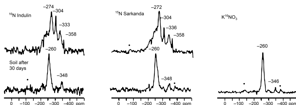
Figure 1. Solid-state ^{15}\text{N} CPMAS NMR spectra of the used ^{15}\text{N} -lignins and the HF-treated soils amended with ^{15}\text{N} -lignins and \text{K}^{15}\text{NO}_3 after one month of incubation. Asterisks indicate spinning side bands. The spectra were obtained at the Lehrstuhl für Bodenkunde, TU-München.
