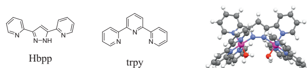
Figure 3. Left: bis(bidentate) Hbpp ligand. Center: ancillary trpy ligand. Right: calculated structure of in, in -{[Ru II (trpy) 2 (H 2 O)] 2 (μ-bpp)} 3+ . Color code: Ru, pink; N, blue; O, red; C, gray; H, white.
