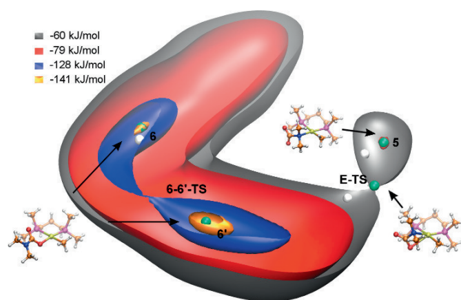
Figure 5. Reconstructed FES of the metadynamic run. The green points denote the minima and the transition state according to the FES. The white points stand for the same structures obtained with QM calculations. The isosurfaces are drawn at the following values: orange ( -141 \text{ kJ mol}^{-1} ), blue ( -128 \text{ kJ mol}^{-1} ), red ( -79 \text{ kJ mol}^{-1} ) and gray ( -60 \text{ kJ mol}^{-1} ).
