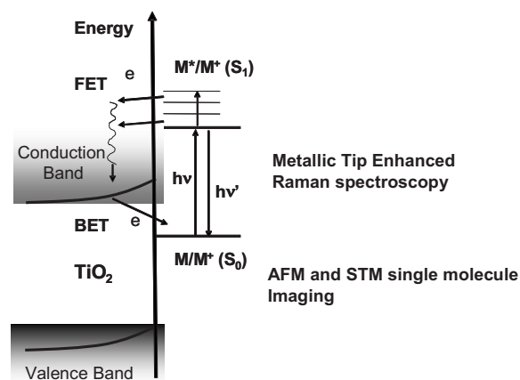
Figure 1. Diagram of interfacial electron transfer processes for the dye-sensitized \text{TiO}_2 system.
